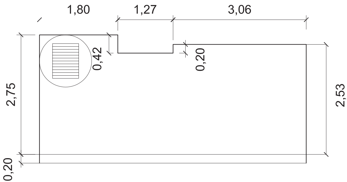
Mezzanine 17 s.m.
