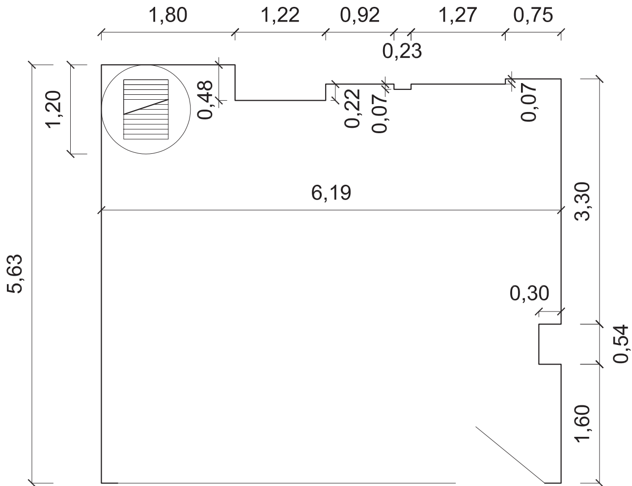
Ground Floor 33 s.m.
